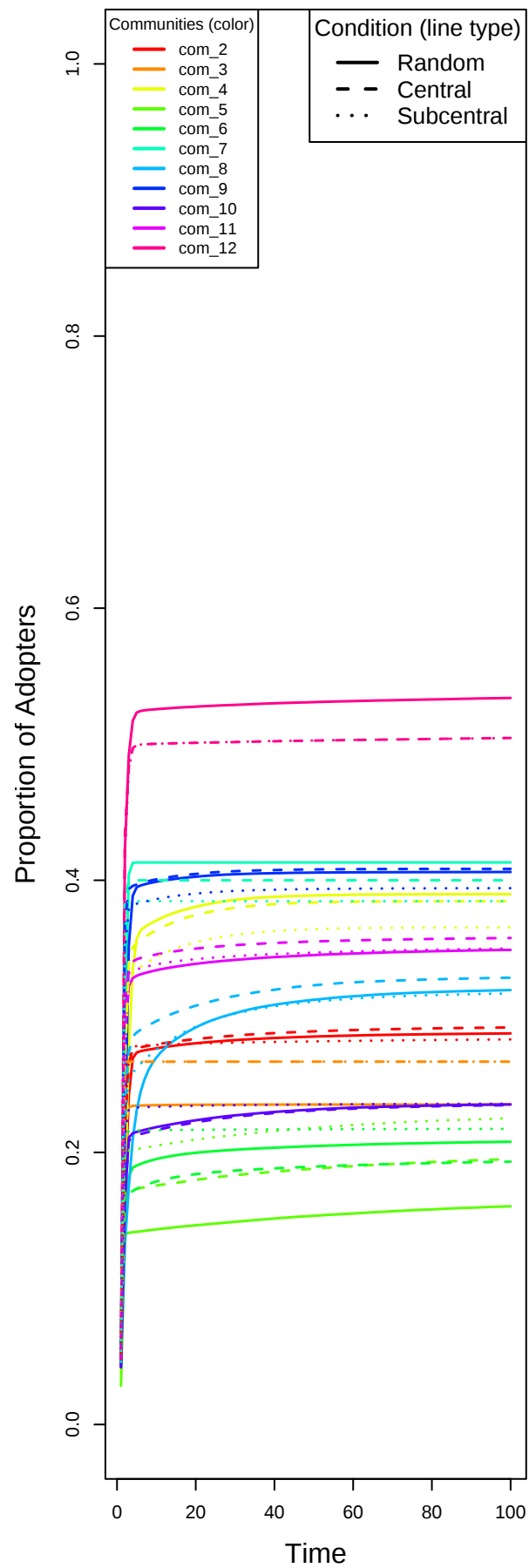
Threshold = Q3
