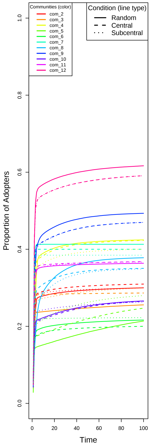
Threshold = M
