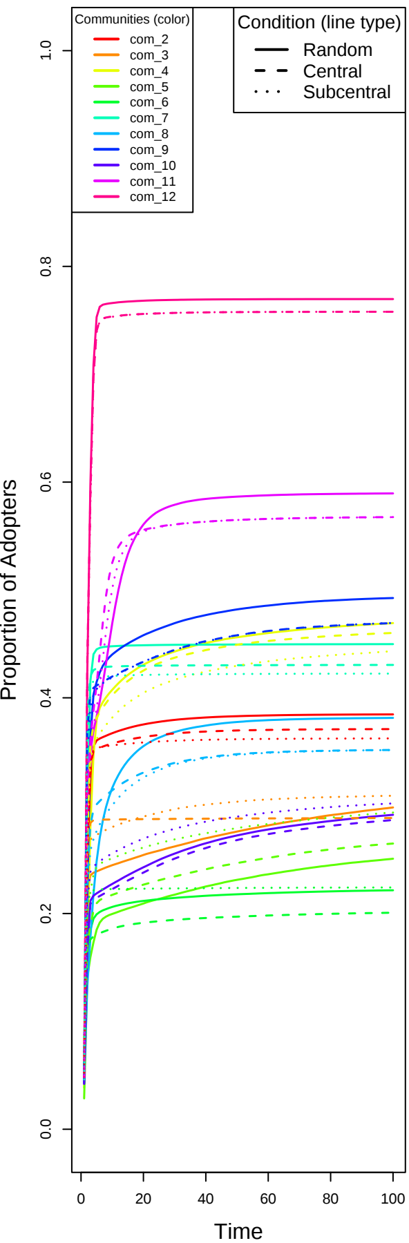
Threshold = Q1
