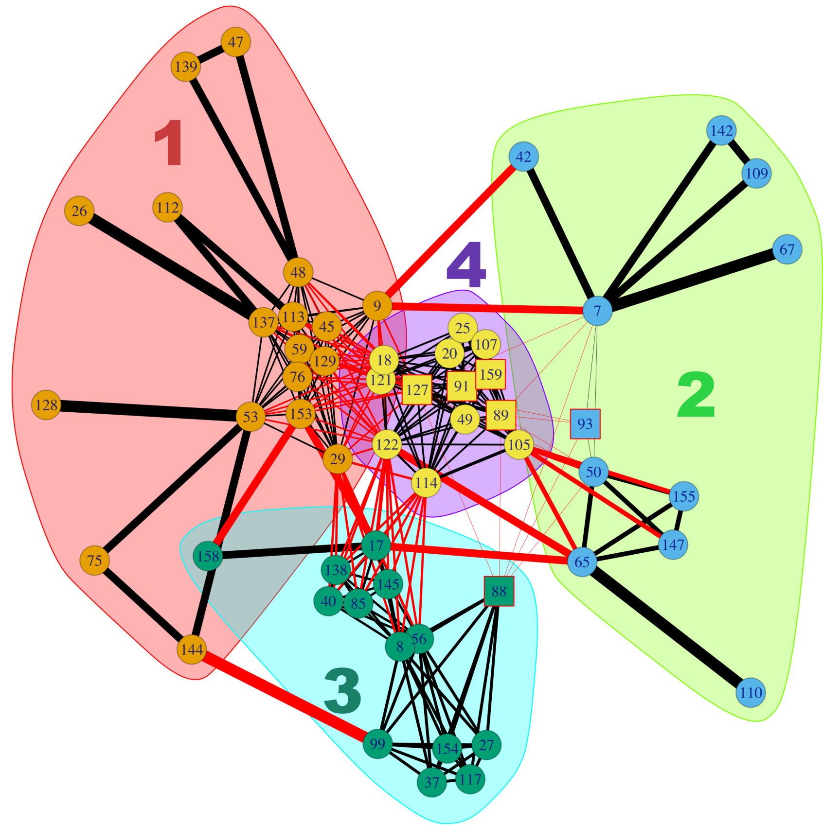
Modularity optimization algorithm with edge weights = membership overlap/proportional club size
